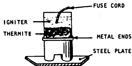
HOLE BURNING METHOD
