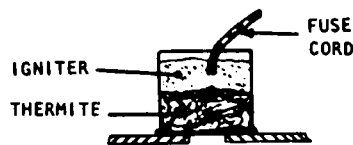
PLATE WELDING METHOD
